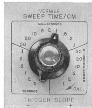
Fig. 4. To simplify sweep selection, sweep time selector is a single, direct-reading control. Concentric vernier enables continuous variation between steps.
